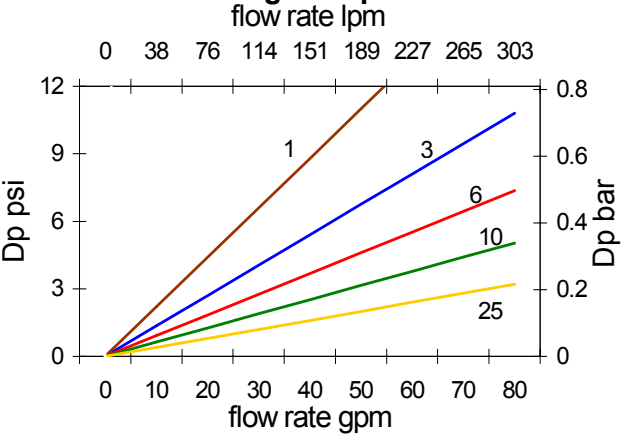
52HL16 Dualglass Dp vs flow rate
