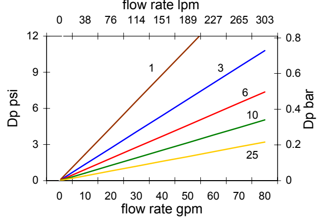
52N/RNL16 Dualglass Dp vs flow rate
