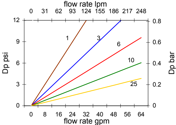
52HL10 Dualglass Dp vs flow rate
