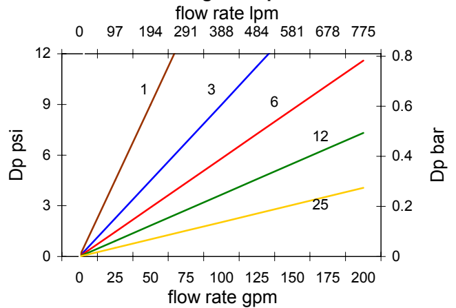
TX3/TL3L19 Dualglass Dp vs flow rate
