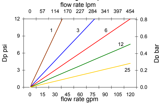
TX3/TL3L11 Dualglass Dp vs flow rate
